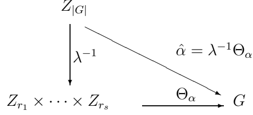
Figure 1: Definition of mapping \hat{\alpha} .
